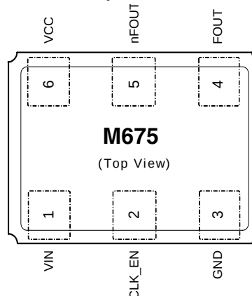
Figure 1: Pin Assignment
