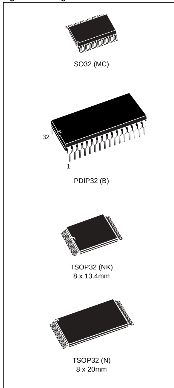
Figure 1. Packages
