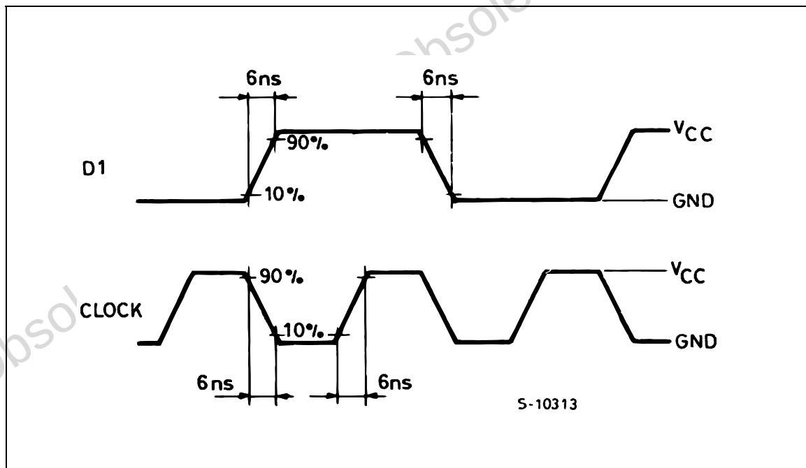
WAVEFORM 4: INPUT WAVEFORMS( f=1\text{MHz} ; 50% duty cycle)
