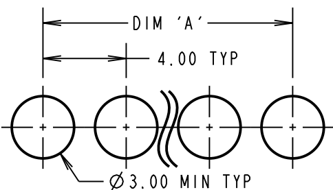
RECOMMENDED PCB LAYOUT FOR M80-33A SMT POWER CONTACTS
