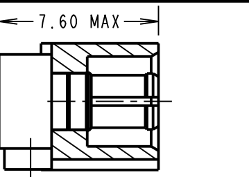
M80-33A x No. OF CONTACTS
