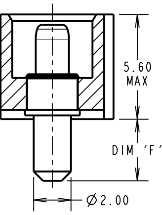
M80-PM1/PM2 x No. OF CONTACTS
