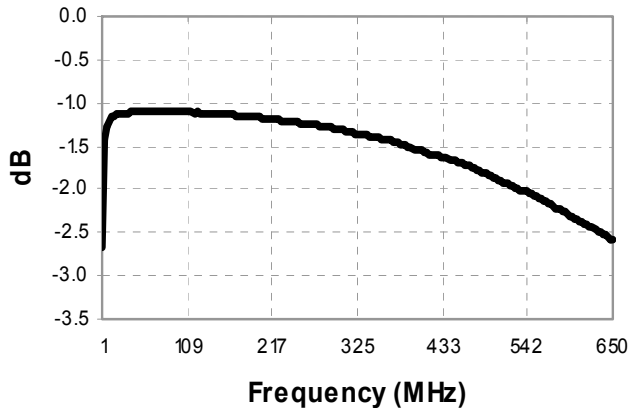
Insertion Loss 1: through pin 4 to pin 3
