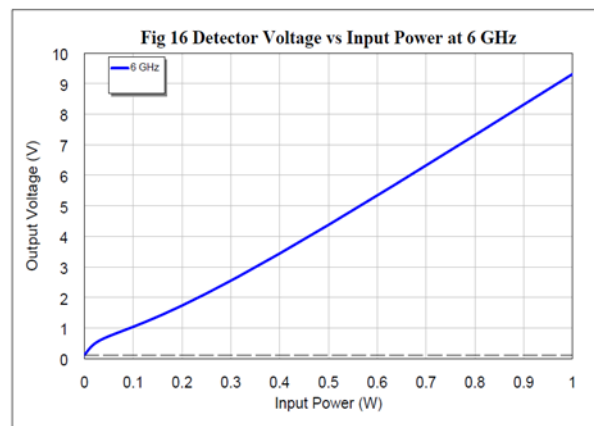
Detector Voltage vs. Input Power (W) @ 6 GHz
