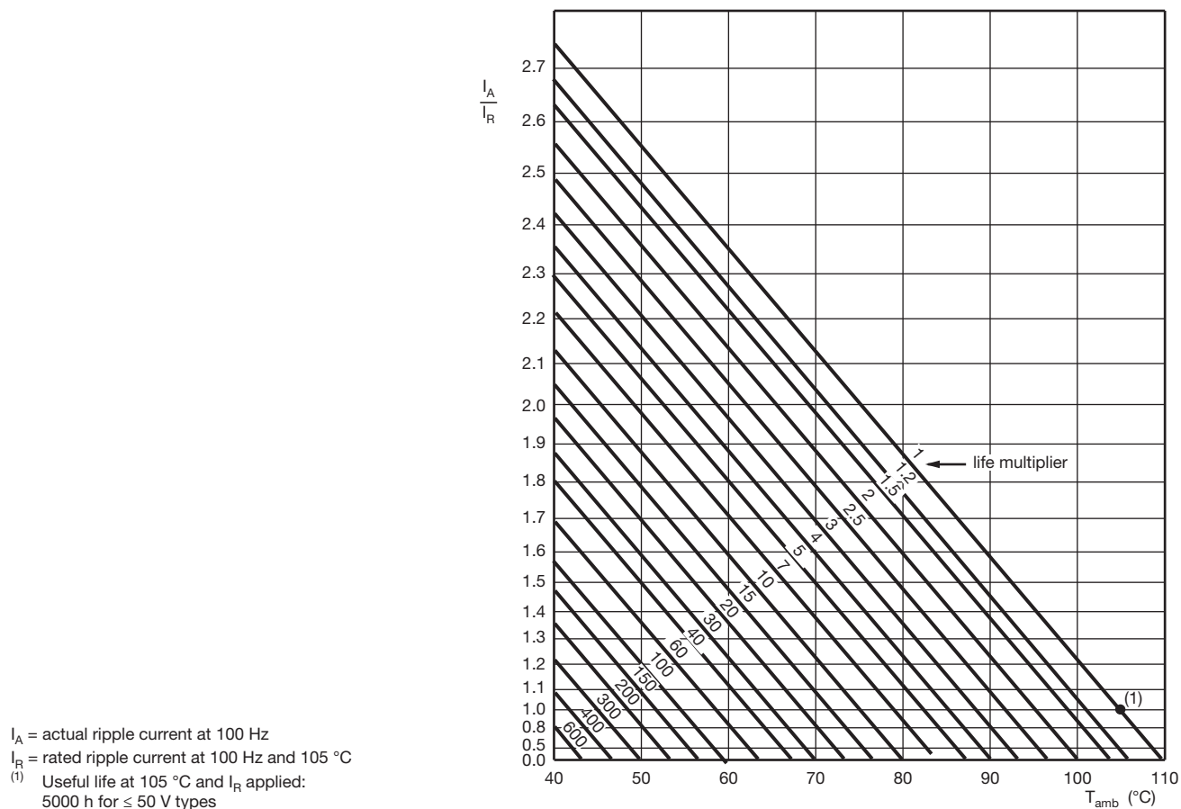
Fig. 18 - Multiplier of useful life as a function of ambient temperature and ripple current load
