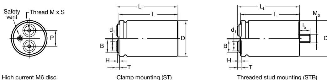
Fig. 2B - Mechanical drawings for high current M6 disc versions. For details refer to Table 2
