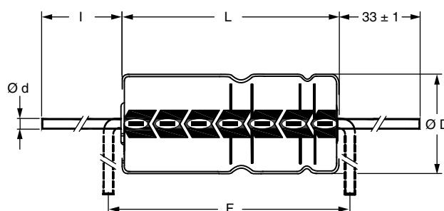
Form AA: Axial in box
