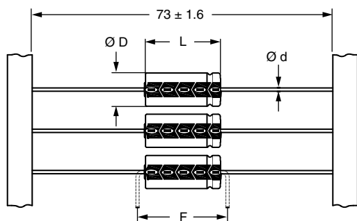
Form BR: Taped on reel
