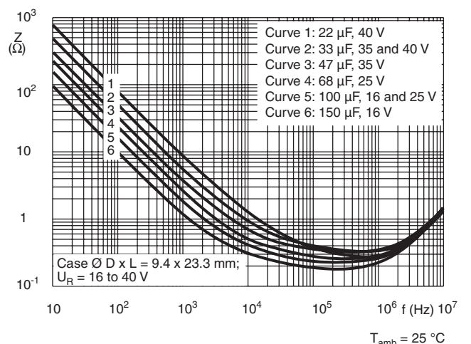
Fig.15 Typical impedance as a function of frequency
