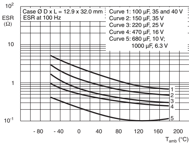
Fig.24 Typical ESR as a function of ambient temperature
