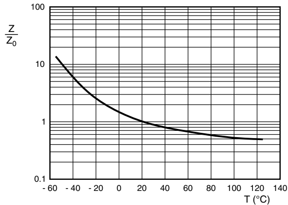
Fig. 9 Typical multiplier of impedance at 100 Hz as a function of temperature ( Z_0 = Z at 20 °C)
