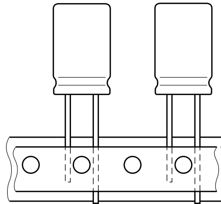
Fig.4 Form TFA: Taped in box (ammpack)
