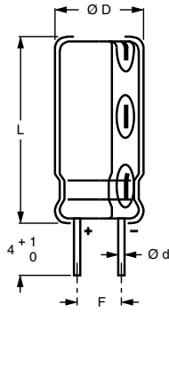
Fig.3 Form CB: Cut leads
