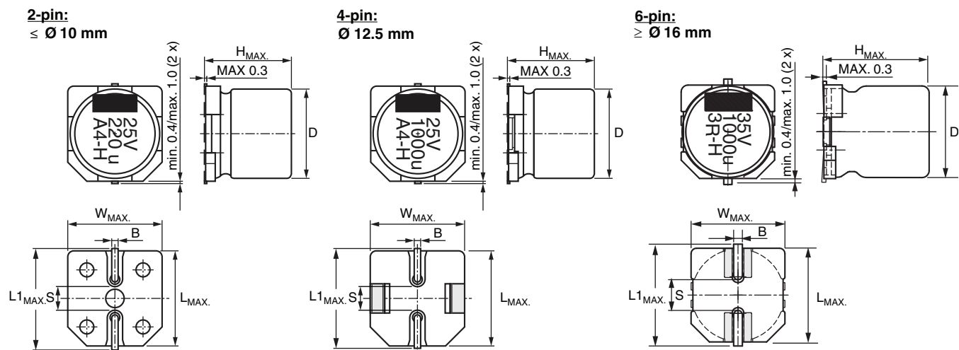
Fig. 2 - Dimensional outline
