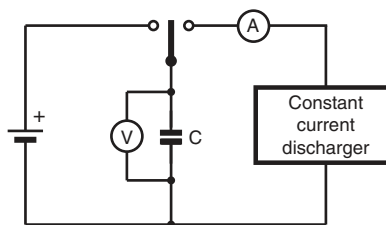
Fig. 16 - Test Circuit for Capacitance Measurement
