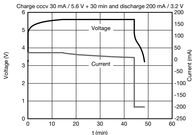
Fig. 29 - Constant Current (CC)-Constant Voltage (CV) Charging Method at RT Typical Charge / Discharge Characteristics at RT: 45 F / 5.6 V
