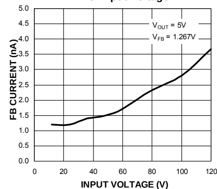
FB Current vs. Input Voltage
