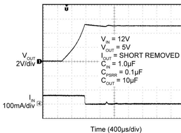
Short-Circuit Output Voltage Recovery
