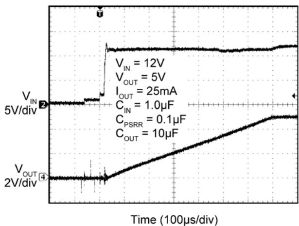
Hot Plug
