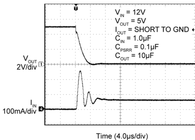
Short-Circuit Response
