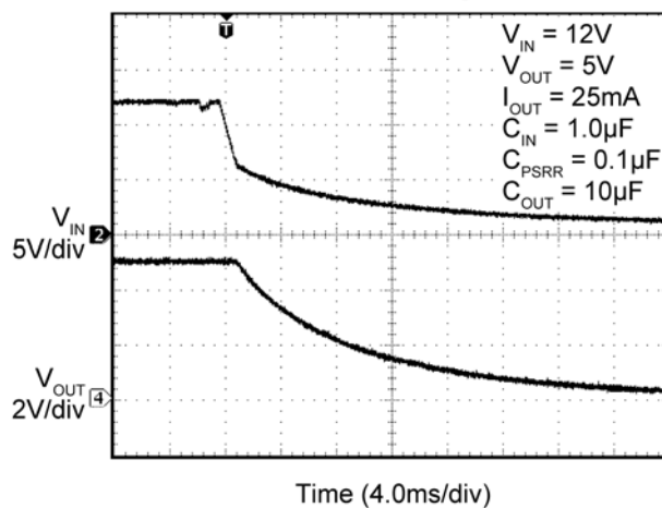
Hot Un-Plug
