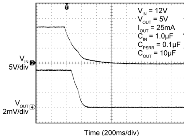
Soft Turn-Off
