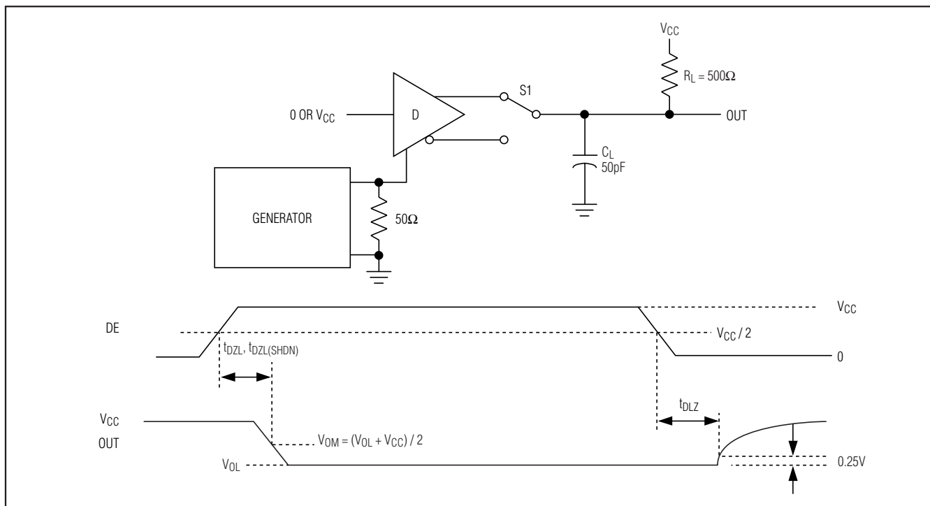
Figure 5. Driver Enable and Disable Times ( t_{DLZ} , t_{DLZ(SHDN)} , t_{DLH} , t_{DLH(SHDN)} )
