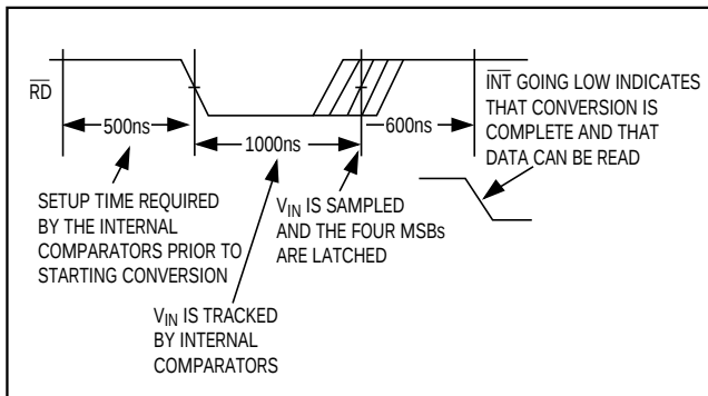
Figure 4. Operating Sequence
