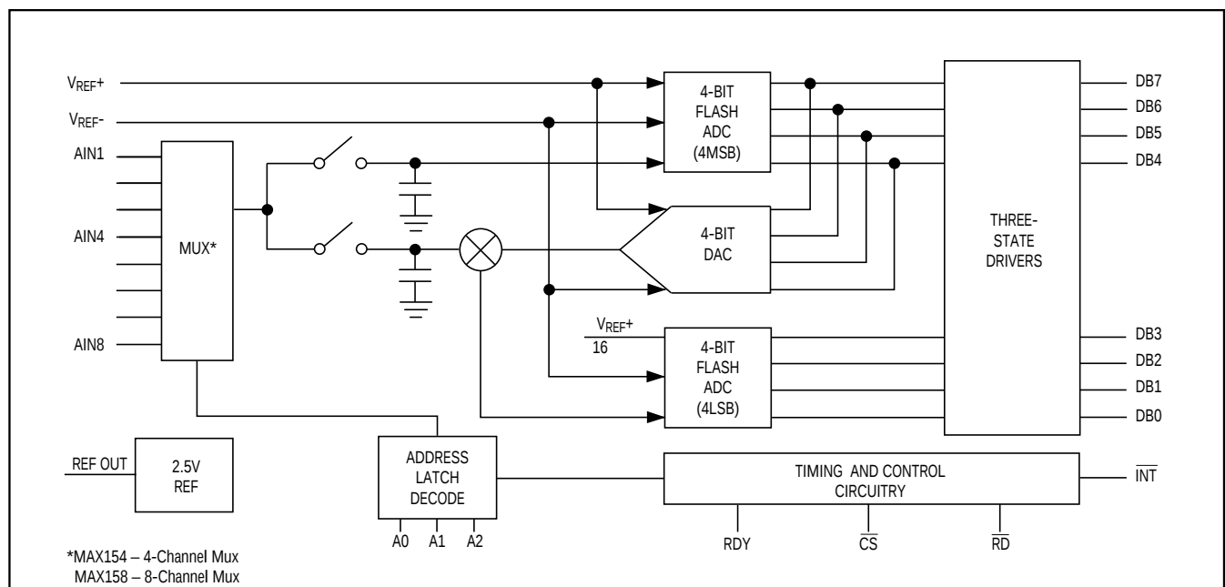
Figure 3. Functional Diagram
