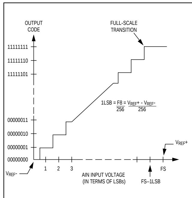
Figure 7. Transfer Function
