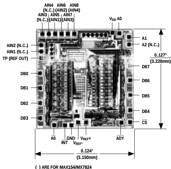
Chip Topography
