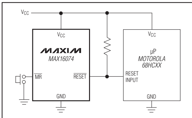
Figure 2. Interfacing to μP with Bidirectional Reset Pins
