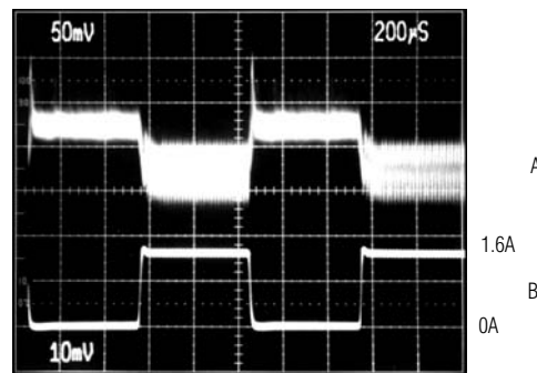
MAX1649 LOAD-TRANSIENT RESPONSE
