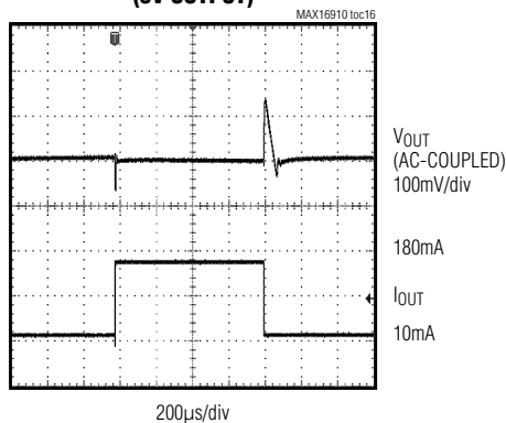
LOAD-TRANSIENT RESPONSE (3V OUTPUT)
