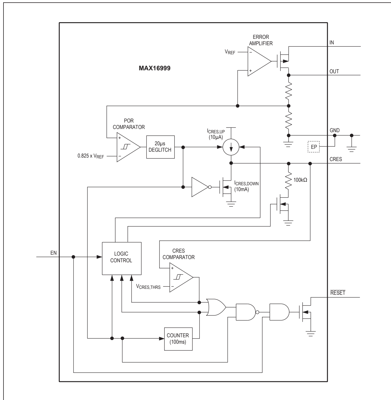
Figure 1. Block Diagram
