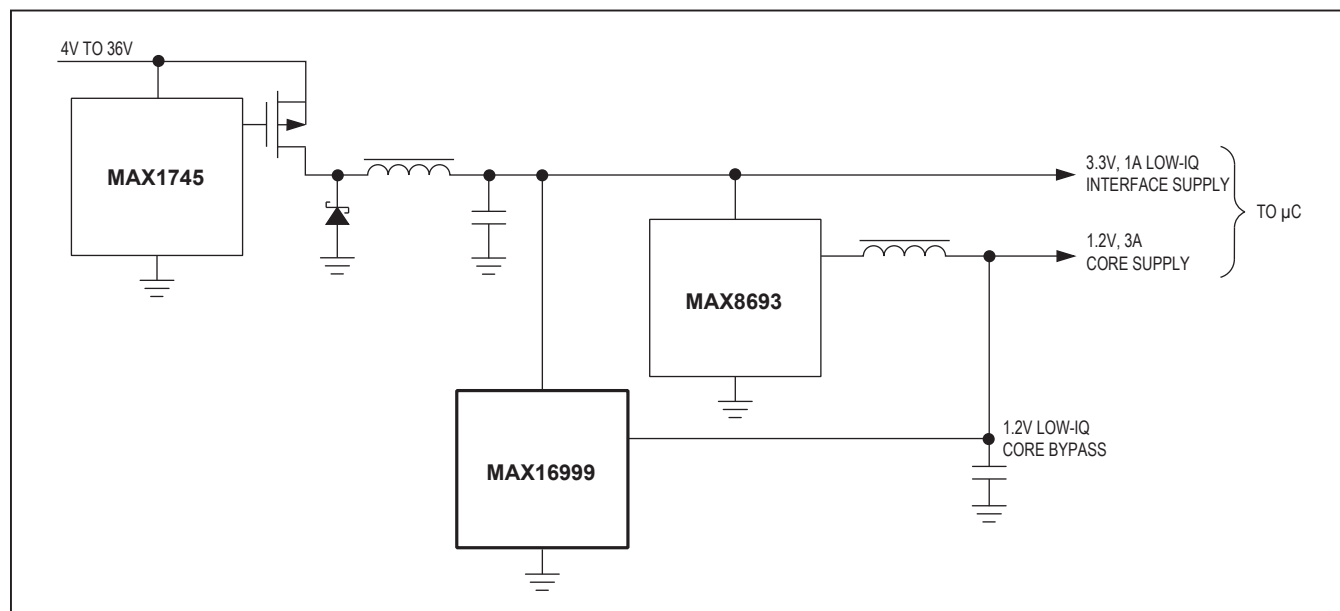
Figure 2. Low-Quiescent \mu\text{C} Supply Solution
