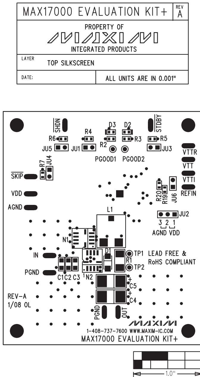
Figure 2. MAX17000 EV Kit Component Placement Guide—Component Side
