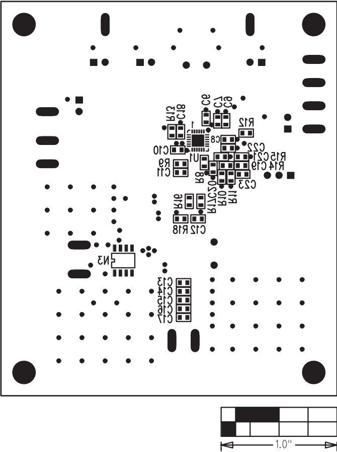
Figure 7. MAX17000 EV Kit Component Placement Guide—Solder Side
