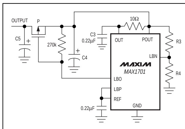
Figure 8. Using the Low-Battery Comparator for Load Control During Start-Up
