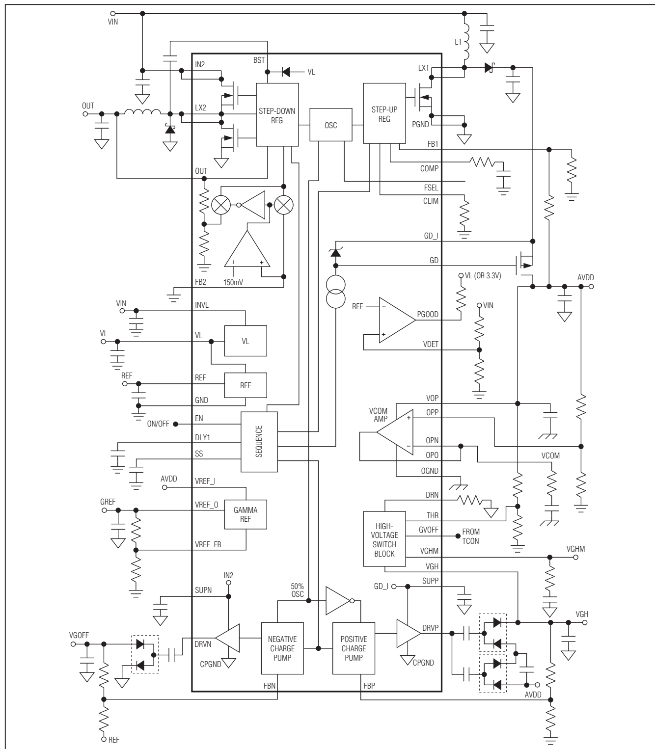
Figure 2. Functional Diagram
