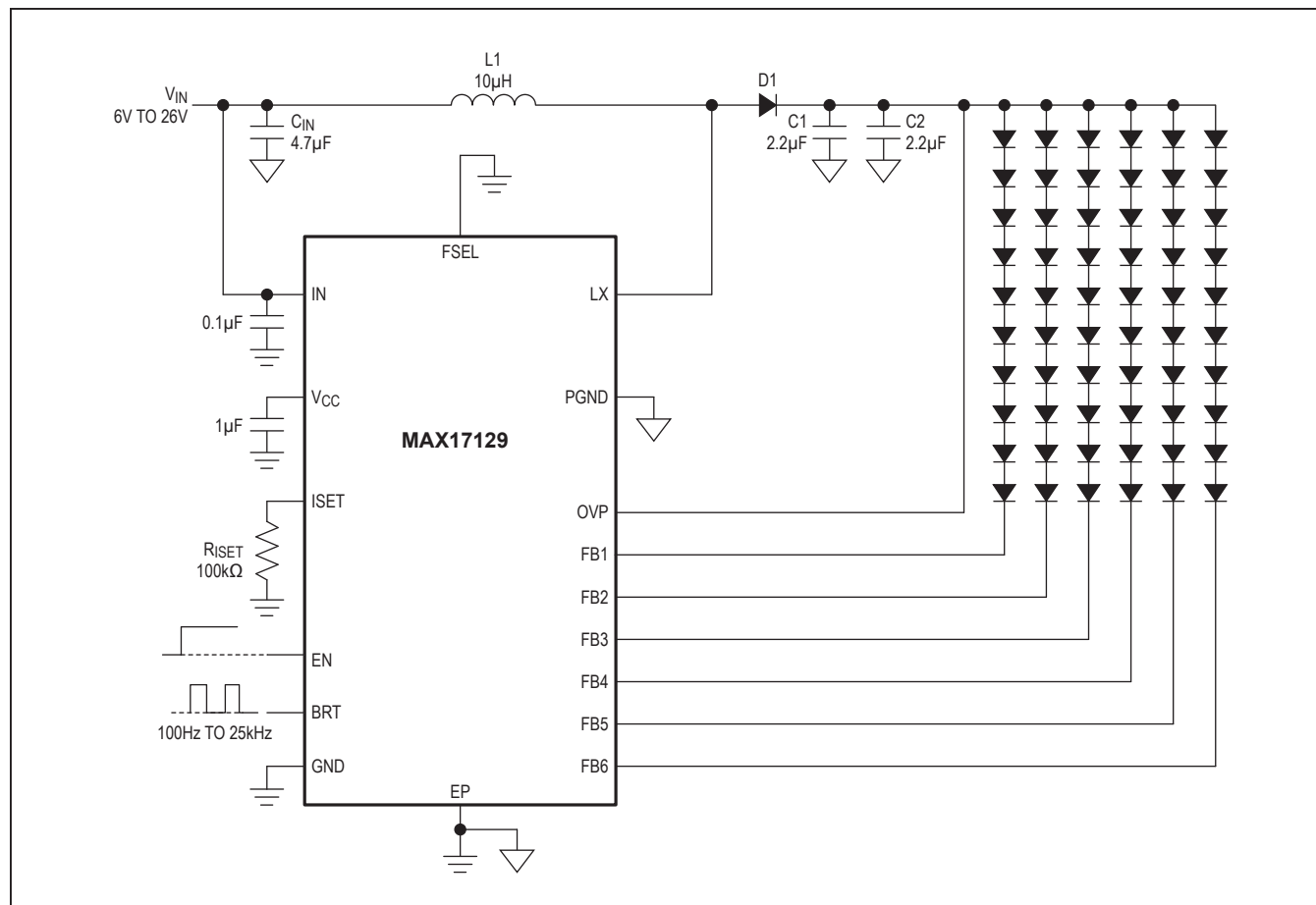
Figure 1. MAX17129 Typical Operating Circuit
