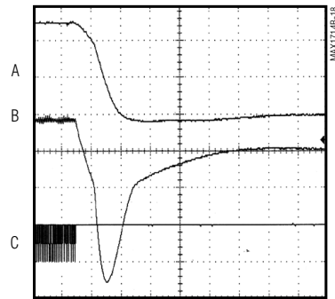
SHUTDOWN WAVEFORM (4A COMPONENTS, V_{OUT} = 2.5V , 300kHz)
