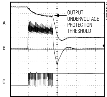
OUTPUT OVERLOAD WAVEFORM (4A COMPONENTS, V_{OUT} = 2.5V , 300kHz)
