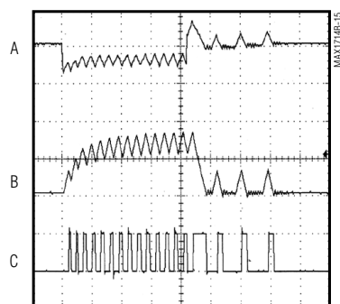
LOAD-TRANSIENT RESPONSE (1.5A COMPONENTS, V_{IN} = 5V , V_{OUT} = 2.5V , 600kHz)
