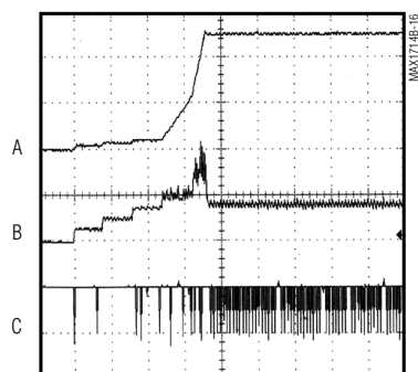
START-UP WAVEFORM (4A COMPONENTS, I_{OUT} = 4A , ACTIVE LOAD, V_{OUT} = 2.5V , 300kHz)
