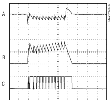
LOAD-TRANSIENT RESPONSE (8A COMPONENTS, V_{OUT} = 1.6V , 300kHz)
