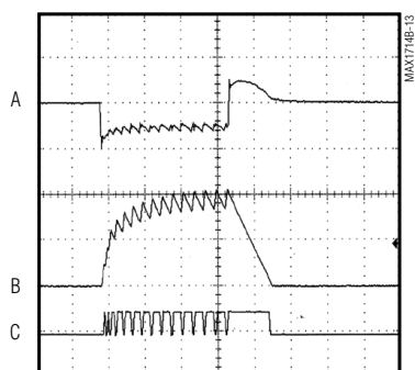
LOAD-TRANSIENT RESPONSE (4A COMPONENTS, V_{OUT} = 2.5V , 300kHz)
