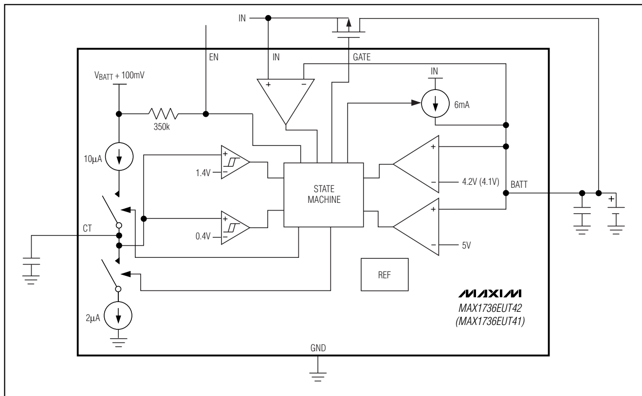
Figure 1. Functional Diagram
