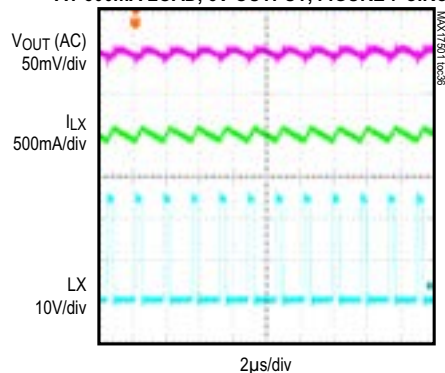
SWITCHING WAVEFORMS OF MAX17501F AT 500mA LOAD, 5V OUTPUT, FIGURE 7 CIRCUIT
