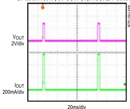
OUTPUT OVERLOAD PROTECTION OF MAX17501F, 5V OUTPUT, FIGURE 7 CIRCUIT
