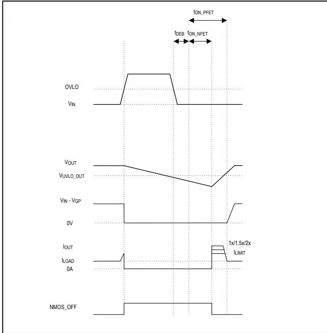
Figure 8. Overvoltage Fault Timing Diagram
