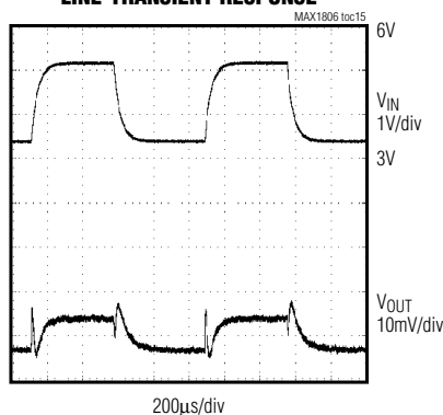
LINE-TRANSIENT RESPONSE
