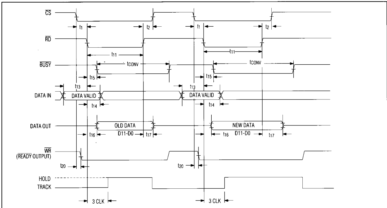
Figure 9a. ROM Mode timing, parallel read ( \text{MODE} = 0 , \text{HBEN} = 0 ).
