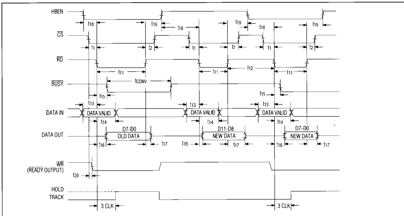
Figure 9b. ROM Mode timing, two-byte read ( \text{MODE} = 0 ).
