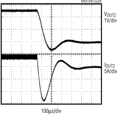
SHUTDOWN WAVEFORM (4A COMPONENTS, \overline{SKIP} = GND , V_{OUT2} = 2.5V )
