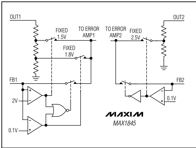
Figure 8. Feedback Mux
