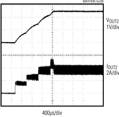
STARTUP WAVEFORM (4A COMPONENTS, \overline{SKIP} = GND , V_{OUT2} = 2.5V )
