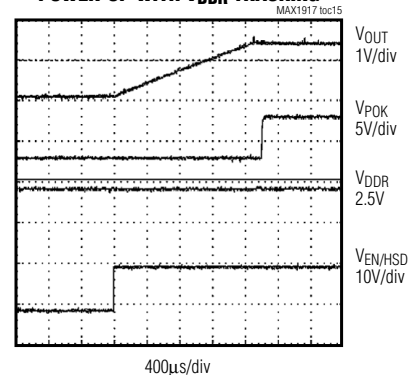
POWER-UP WITH VDD TRACKING
