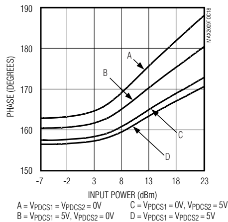
PHASE EXPANSION vs. INPUT POWER
