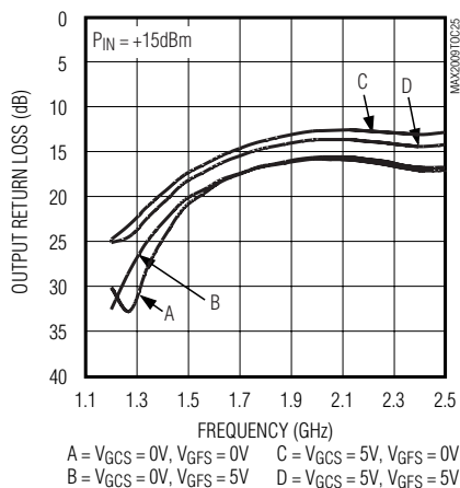
LARGE-SIGNAL OUTPUT RETURN LOSS vs. FREQUENCY
