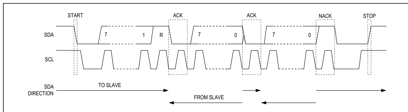
Figure 23. Read Transaction
