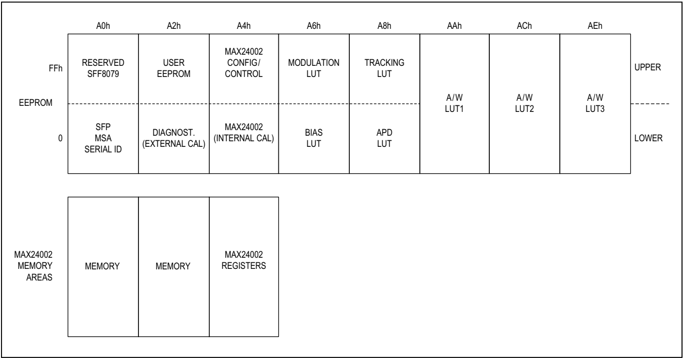
Figure 18. Address Map
