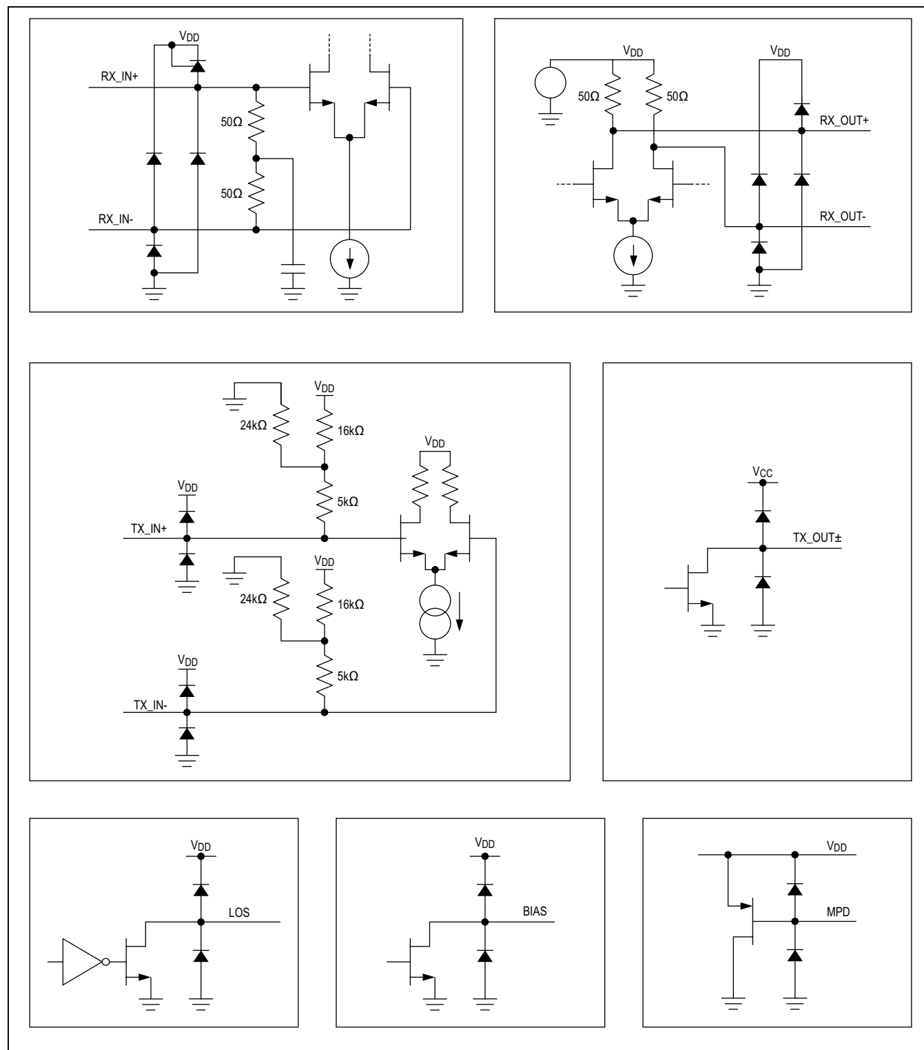
Figure 24. Interface Diagrams
