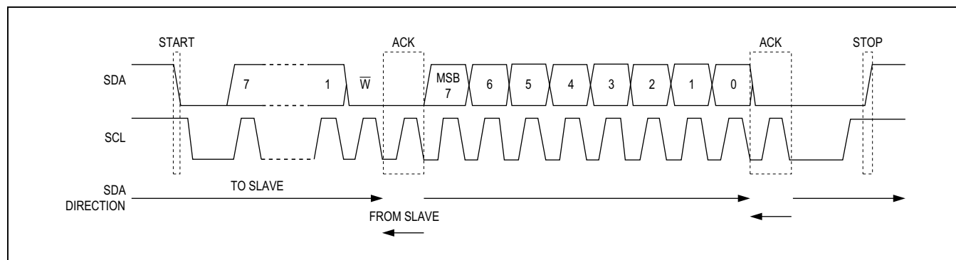
Figure 22. Write Transaction
