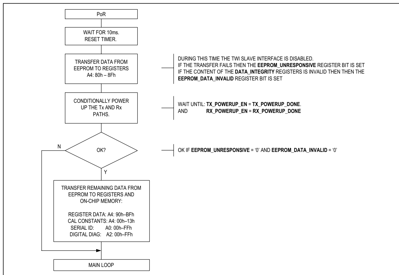
Figure 19. Initialization Sequence
