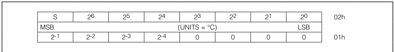
Figure 5. Temperature, T HIGH , and T LOW Register Format
