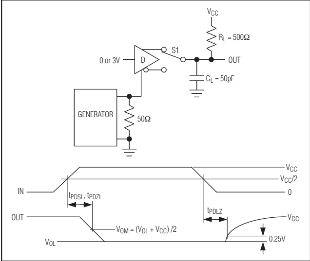
Figure 4. Driver Enable and Disable Times ( t_{PDSL} , t_{PDSL} , t_{PDLZ} )
