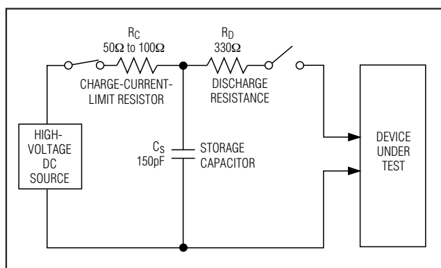
Figure 9. IEC 1000-4-2 ESD Test Model
