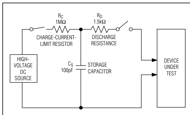
Figure 7. Human Body ESD Test Models
