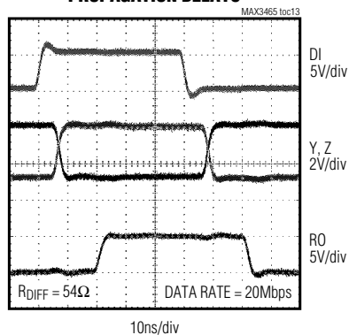
DRIVER AND RECEIVER PROPAGATION DELAYS
