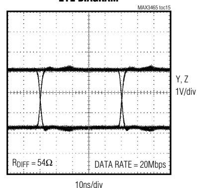
EYE DIAGRAM
