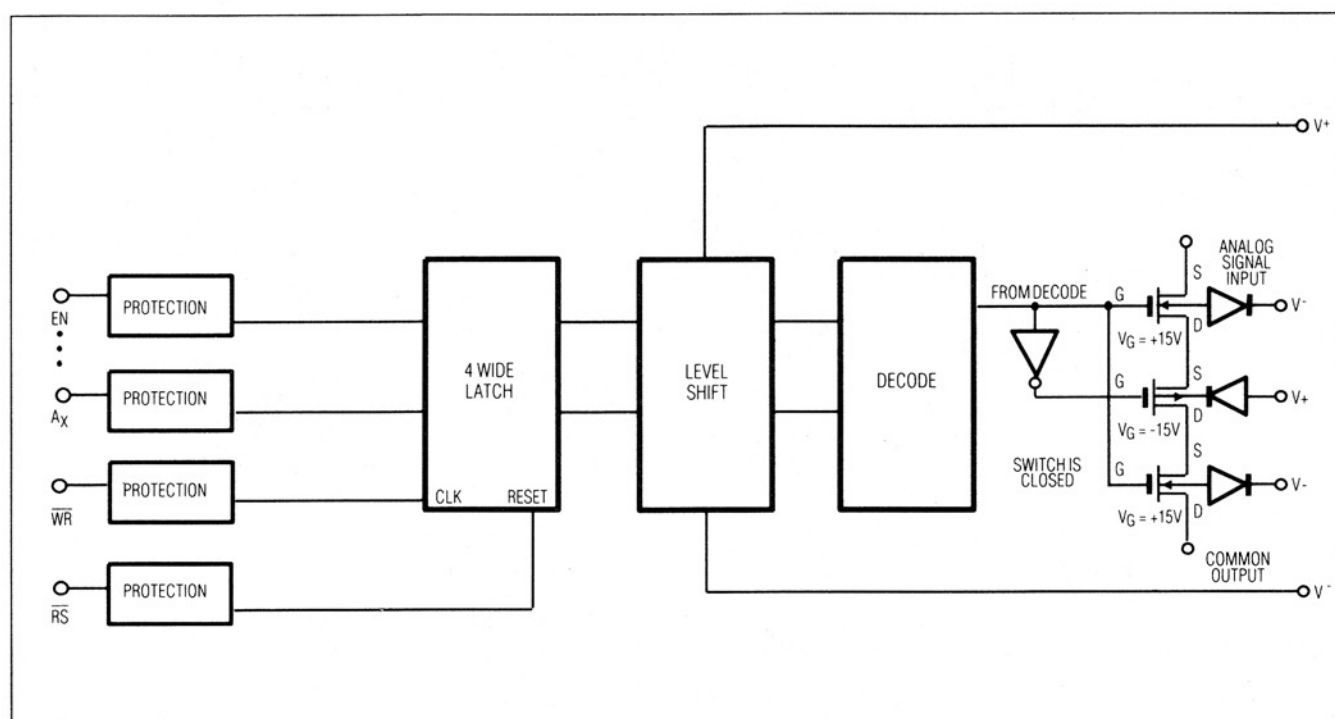
Figure 12. Simplified Internal Structure
