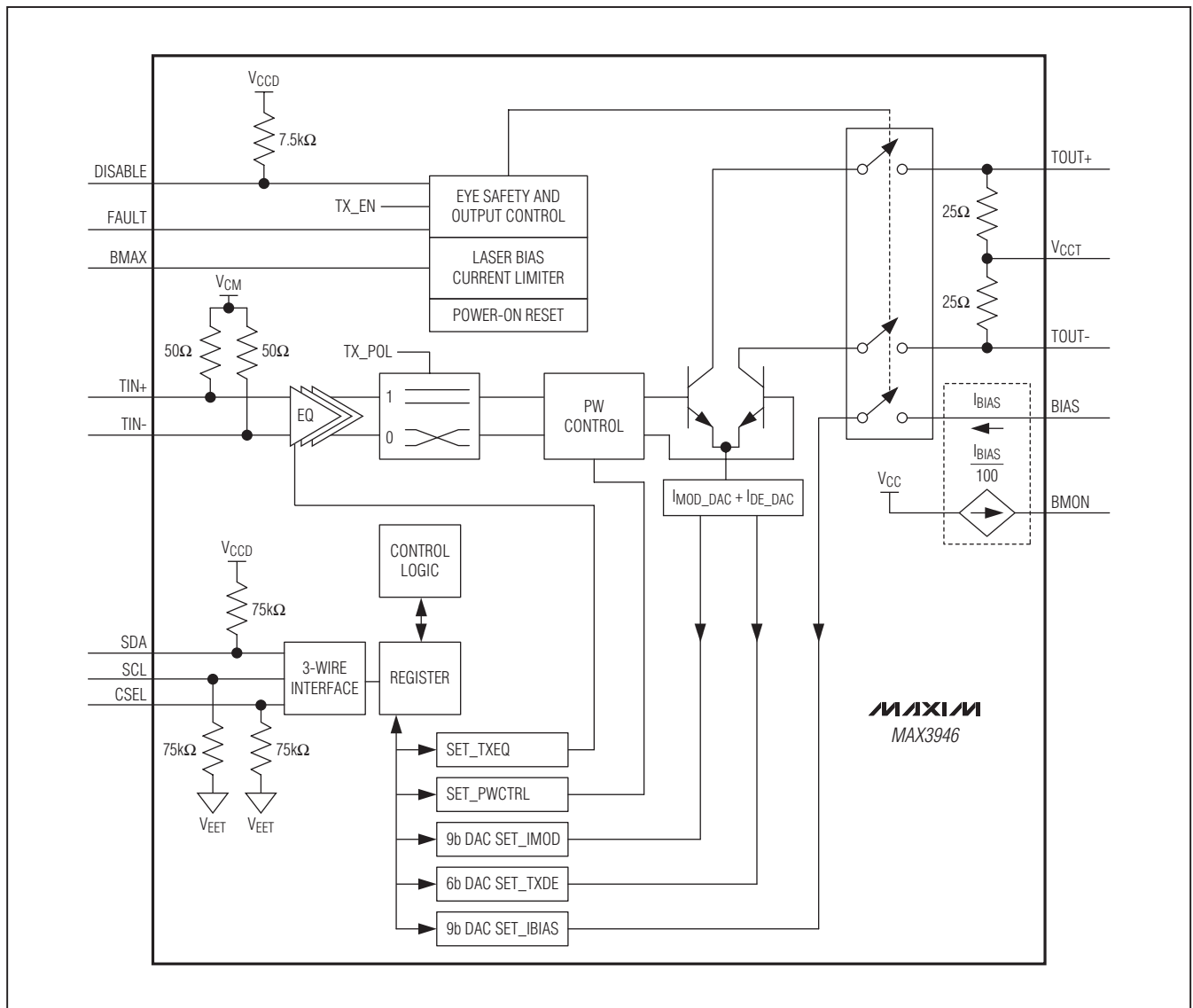
Figure 2. Functional Diagram
