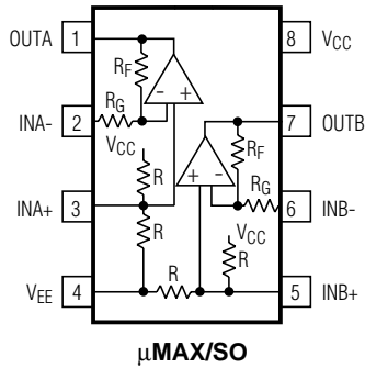
MAXIM MAX4275
