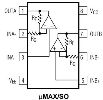
MAXIM MAX4274
