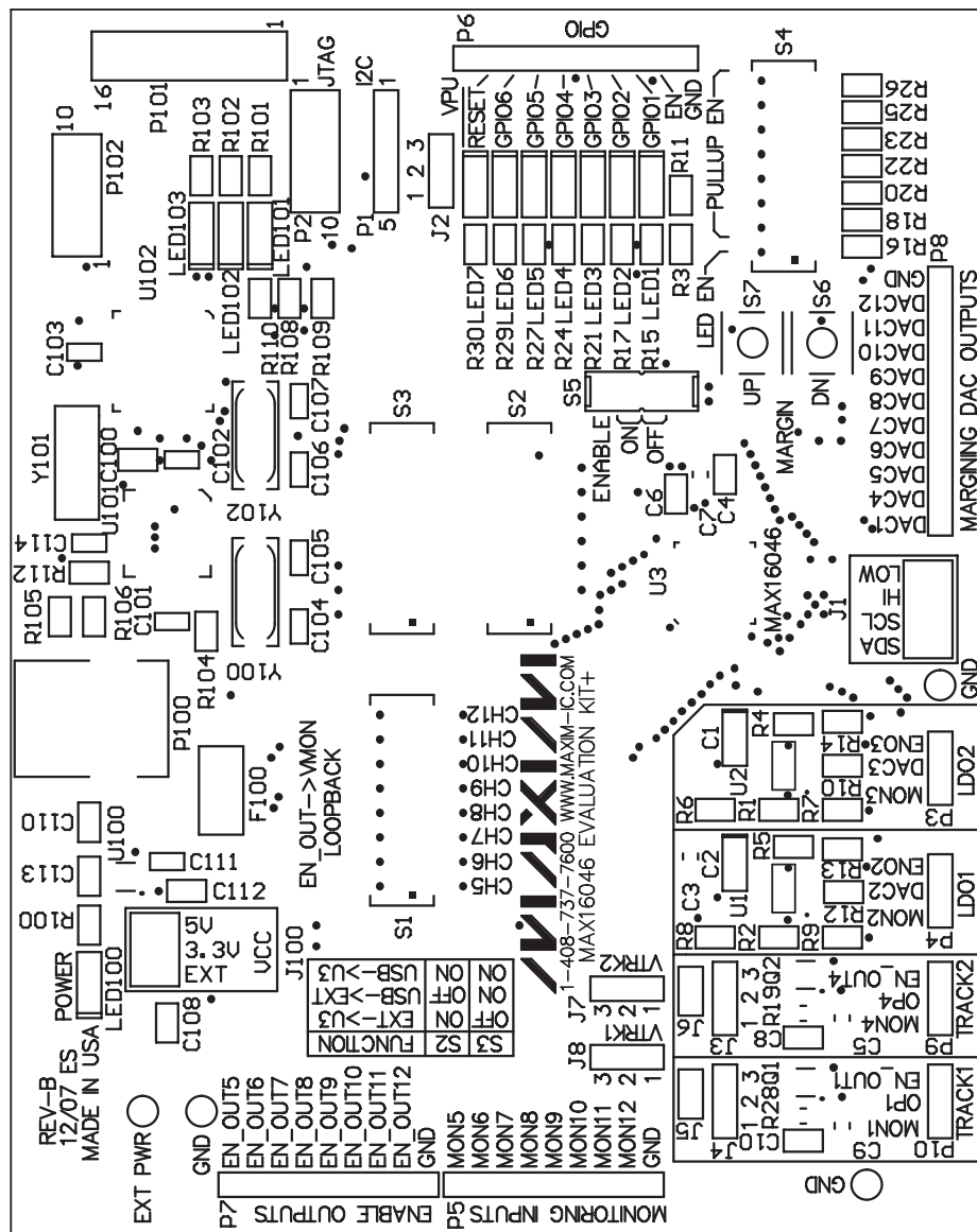
Figure 14. MAX16046 EV Kit Component Placement Guide—Component Side
