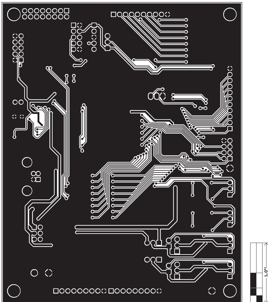
Figure 16. MAX16046 EV Kit PCB Layout—Solder Side
