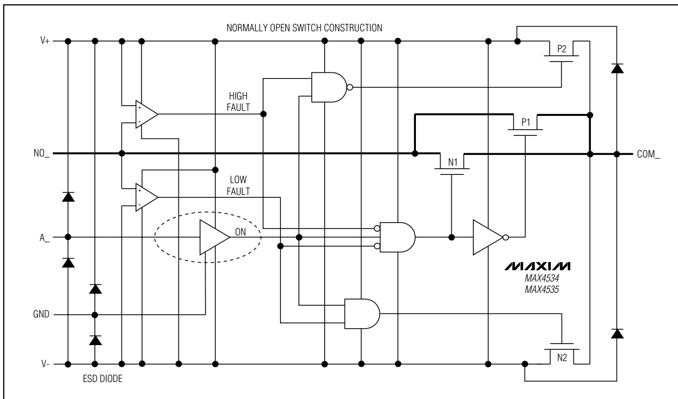
Figure 1. Functional Diagram
