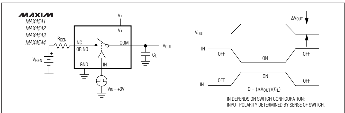
Figure 4. Charge Injection
