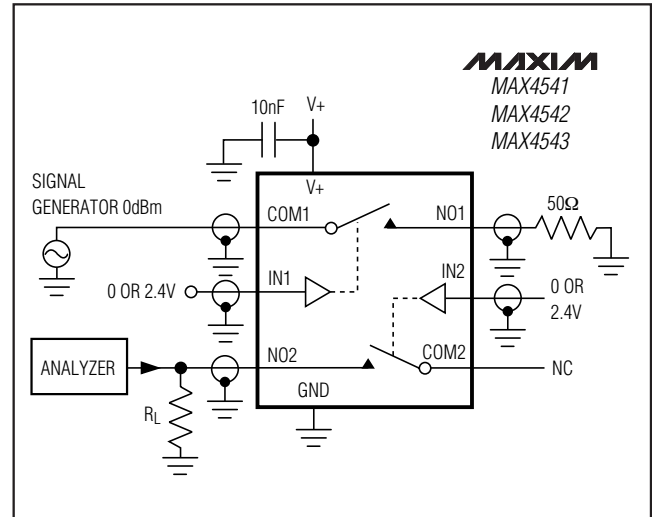
Figure 6. Crosstalk
