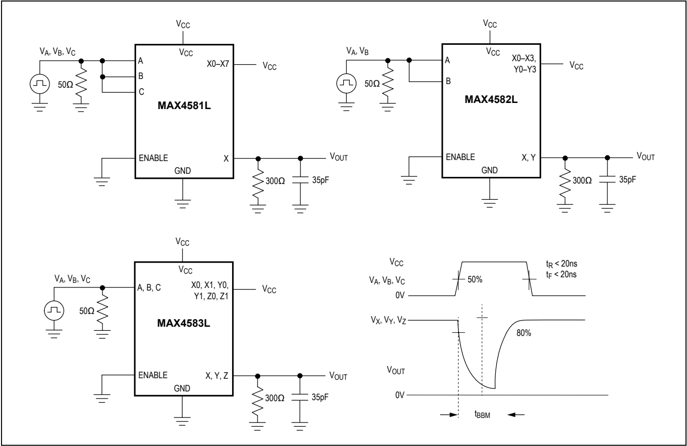
Figure 3. Break-Before-Make Interval
