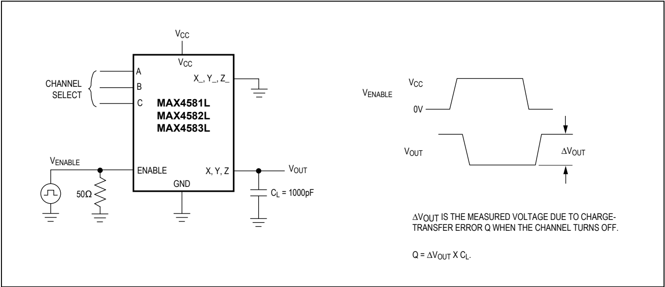
Figure 4. Charge Injection
