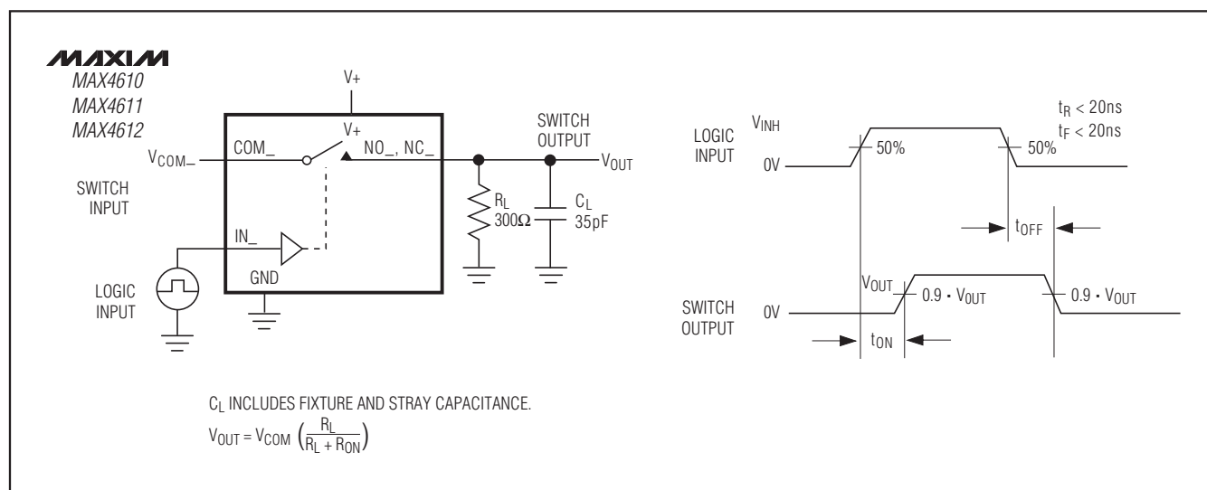
Figure 2. Switching Time
