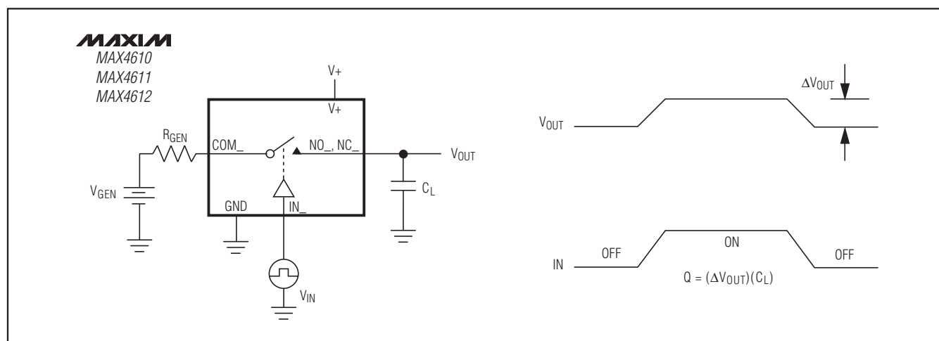
Figure 3. Charge Injection
