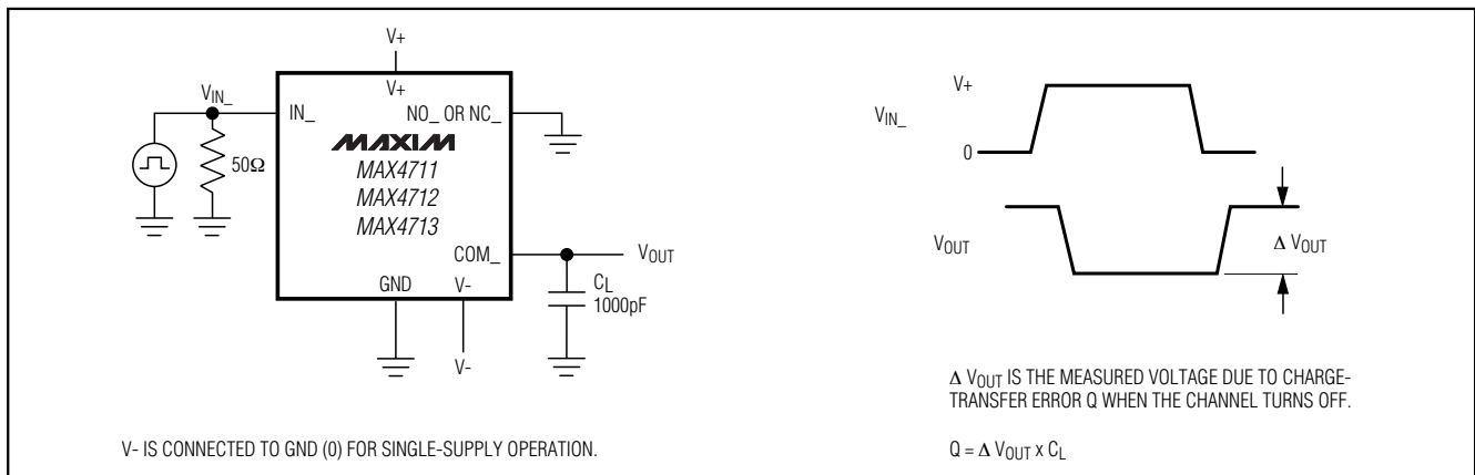
Figure 4. Charge Injection
