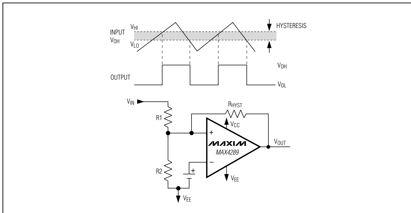
Figure 5. Hysteresis Comparator Circuit
