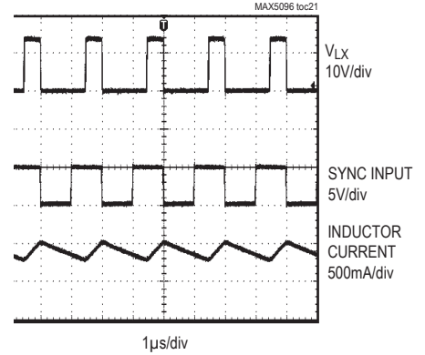
LX VOLTAGE, SYNC INPUT, AND INDUCTOR CURRENT
