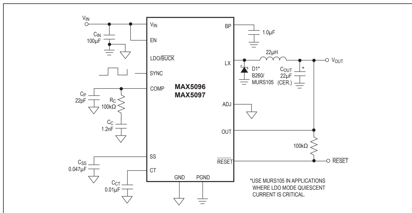
Figure 2. Fixed Output-Voltage Configuration
