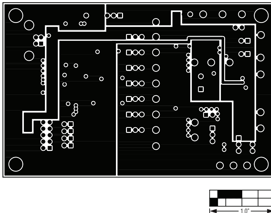
Figure 6. MAX54X EV Kit PCB Layout—Power Layer 3
