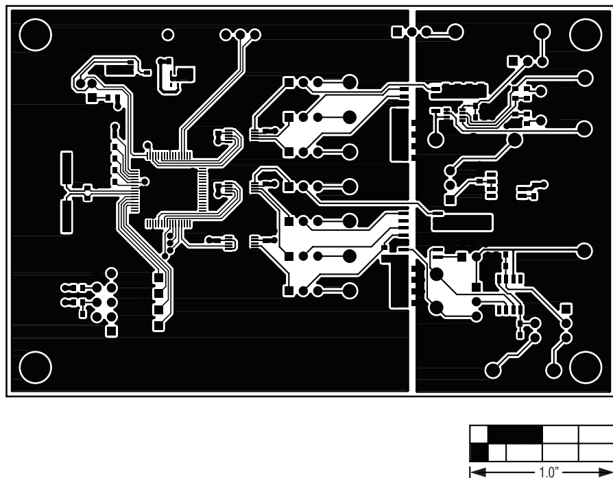
Figure 4. MAX54X EV Kit PCB Layout—Component Side
