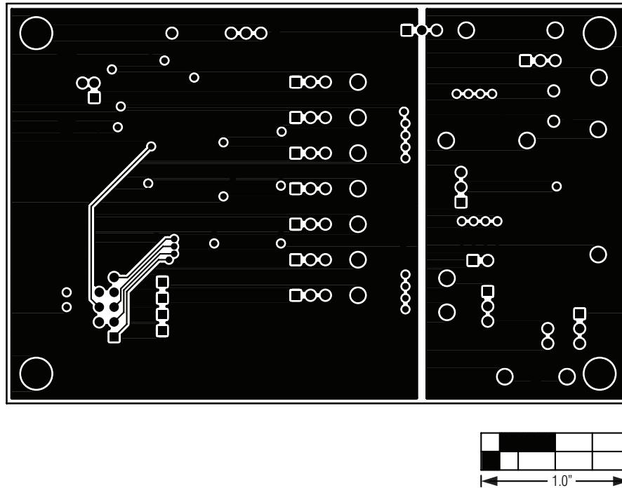
Figure 7. MAX54X EV Kit PCB Layout—Solder Side
