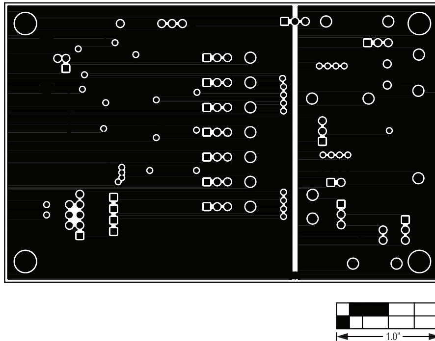
Figure 5. MAX54X EV Kit PCB Layout—Ground Layer 2
