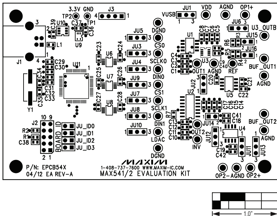
Figure 3. MAX54X EV Kit Component Placement Guide—Component Side
